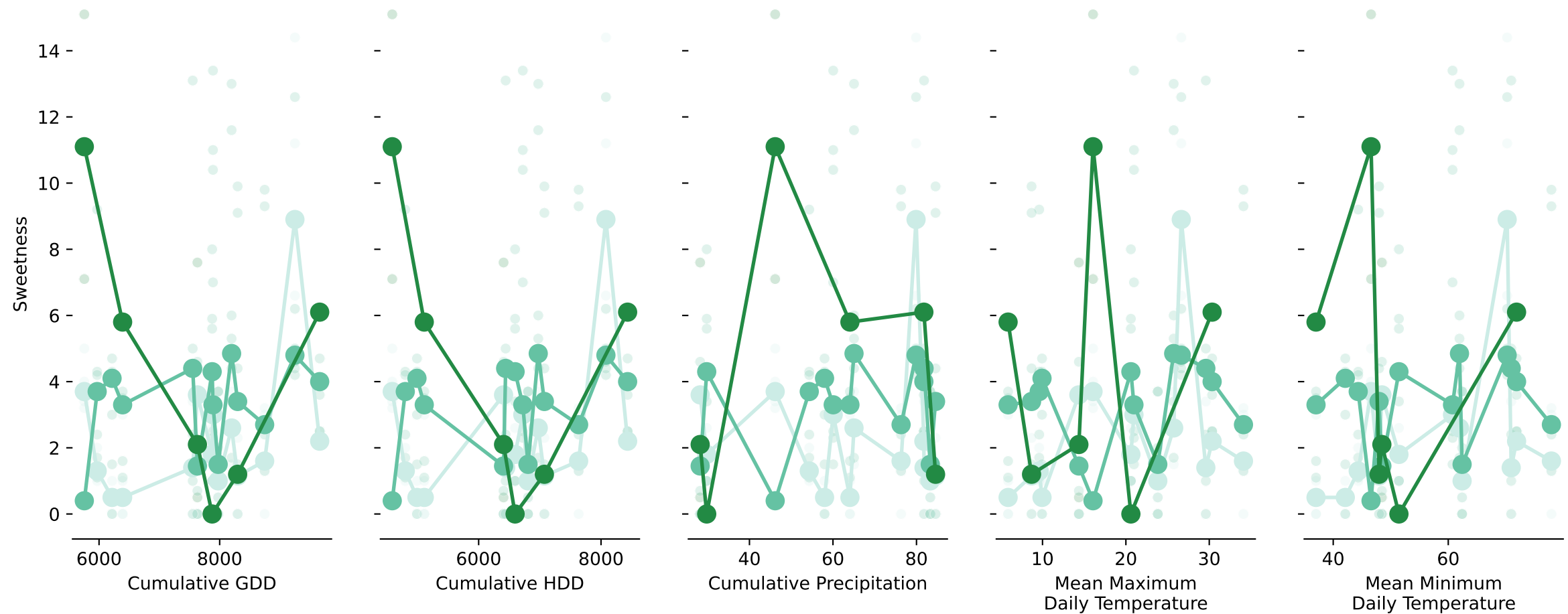
Under Ripe Ripe Over Ripe Climate impacts on Sweetness for Marquette, 2019
